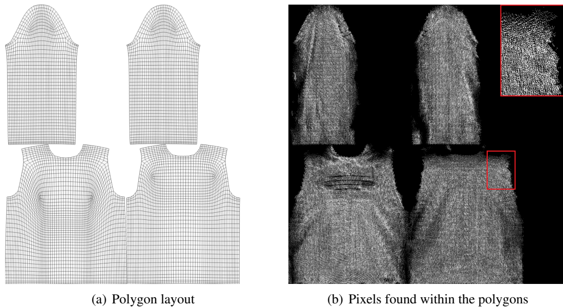
Figure 6.3: UV texture
