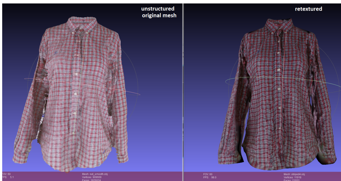
Figure 6.6: Final results
