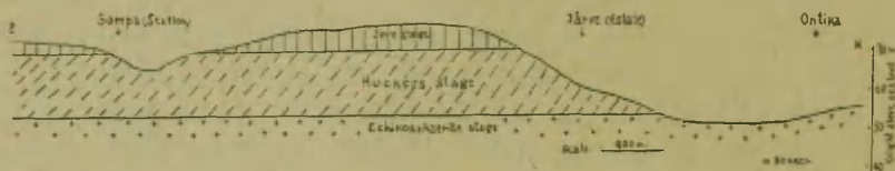
Text fig. 2. Section: Somp—Ontika.
