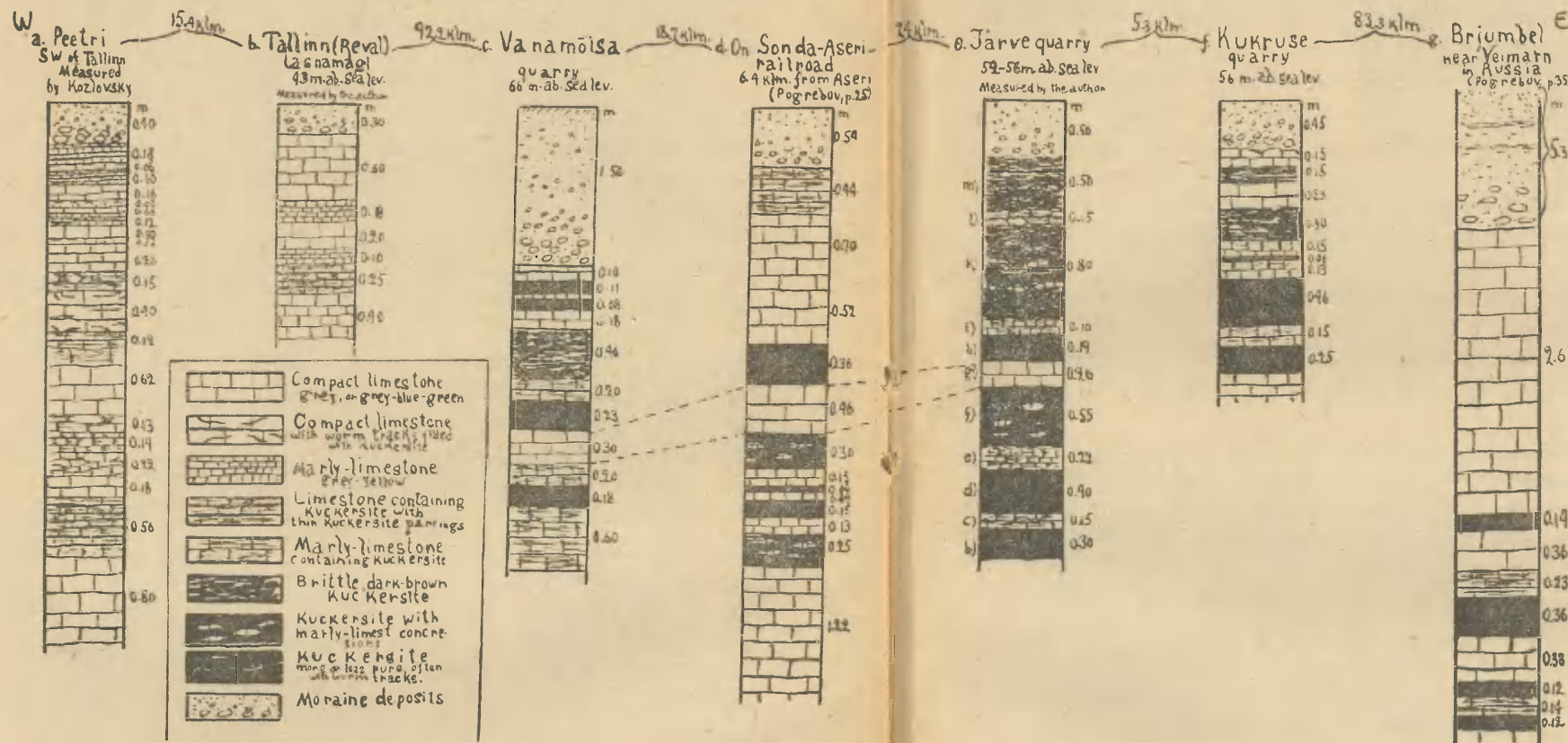
Text fig. 7. Comparative thickness of the kuckersite beds in the Kuckers stage after data of diggings and exposures in quarries.
