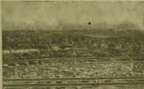
Text fig. 8. Disturbance of limestone and kuckersite beds in the quarry of Kohtla-Järve. Photogr. by J. Ackerberg.
