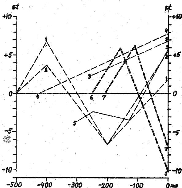
Fig. 1. Average contours of English and Estonian general questions. The thin contours are for good English questions: 1 and 2 from Hadding-Koch and Studdert-Kennedy, 3 - Garding and Abramson, 4- Majewski and Bladell, 5 - Greenberg; the thick lines are for good Estonian questions: 6 - synthetic, 7 - natural.
