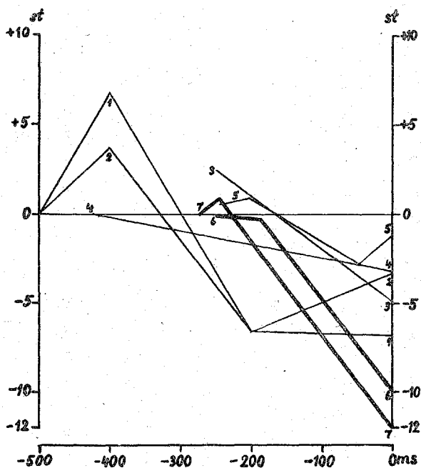
Fig. 2. Average contours of English and Estonian statements. Denotation as in Fig. 1.
