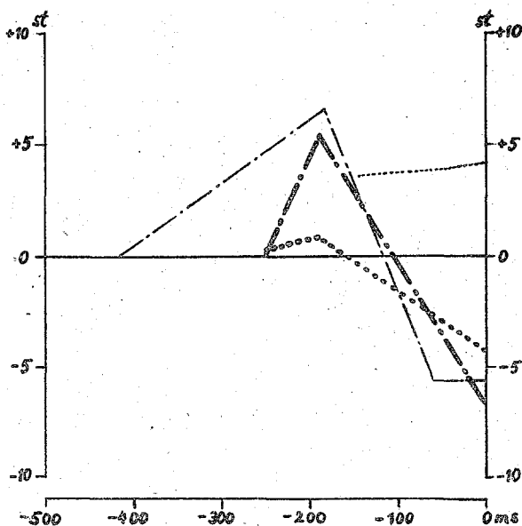
Fig. 3. Average contours of English and Estonian exclamations (dash-and-dot lines) and incomplete utterances (dotted lines). Otherwise denotation as in Fig. 1.
