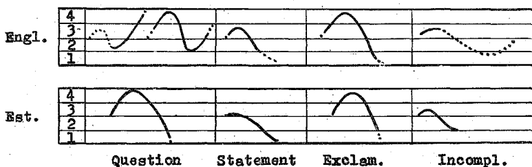
Fig. 4. Generalized pitch contours of four communicative types of utterances in English and Estonian, displayed on four 5-st levels of speakers' overall pitch range.
