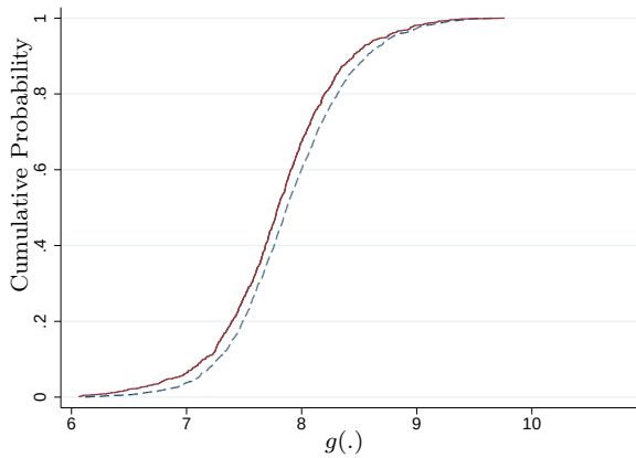
(a) Year-wise average g(\cdot)
