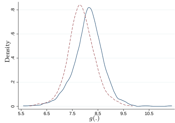
(b) Density plots of g(\cdot)
