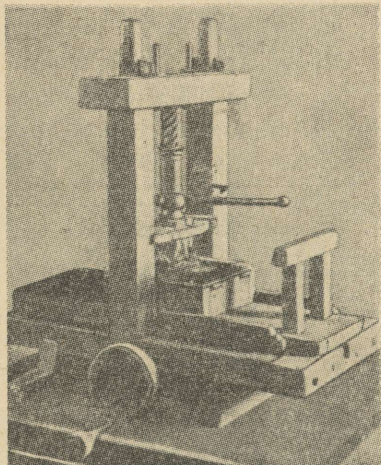
XVI sajandi trükipress. Restauration. Foto.
