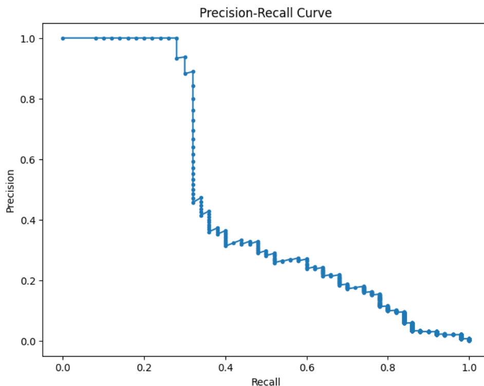
Figure 4.3: Precision-Recall Curve
