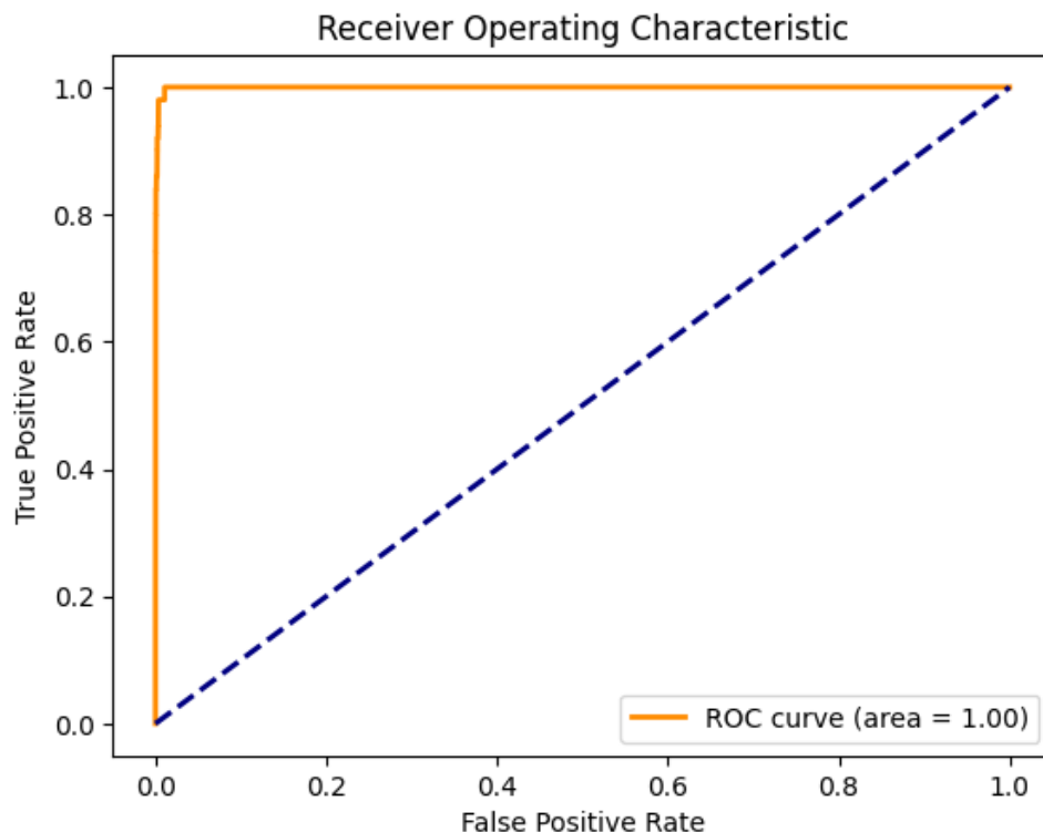
Figure 4.4: Receiver Operating Characteristic Curve (The x-axis represents the false positive rate and the y-axis represents the true positive rate).
