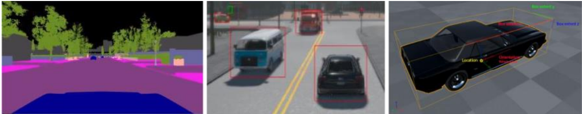
Figure 7. From the left: semantic segmentation, 2D bounding boxes, 3D bounding boxes in CARLA.
