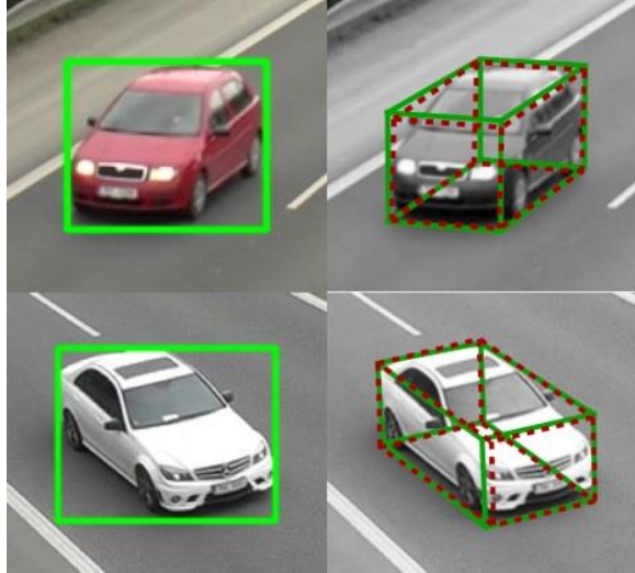
Figure 5. Bounding boxes 2D (left) and 3D (right). 12
