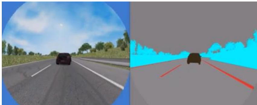
Figure 25. Example images from SCANeR Studio simulation, with semantic segmentation on the right.
