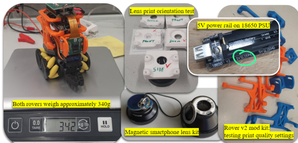
Figure 3.3: Printed part tests & breakout board planning. Rover v1 weighed ~342g. Rover v2's design process focused on the lens mount (top middle), lens placement and camera specifications, ensuring good image quality. A breakout board with a switch was added to control the 18650 PSU (top right) power rail.
