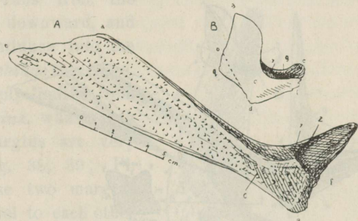
Fig. 37. The antero-lateral plate of Homostius sp. seen from the outside ( A ) compared with the corresponding plate of Dinichthys ( B — strongly reduced). a — upper front angle, a-b — upper margin, a-y — front margin, b — upper hind angle, b-d — hind margin, d-f — lower margin, e — hind wing, f — lower front part, g — upper margin of the hind wing, y — front thickening, z — impression in front of sculptured part.
