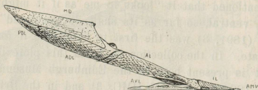
Fig. 44. The same reconstruction as in fig. 43 seen from the right side.
