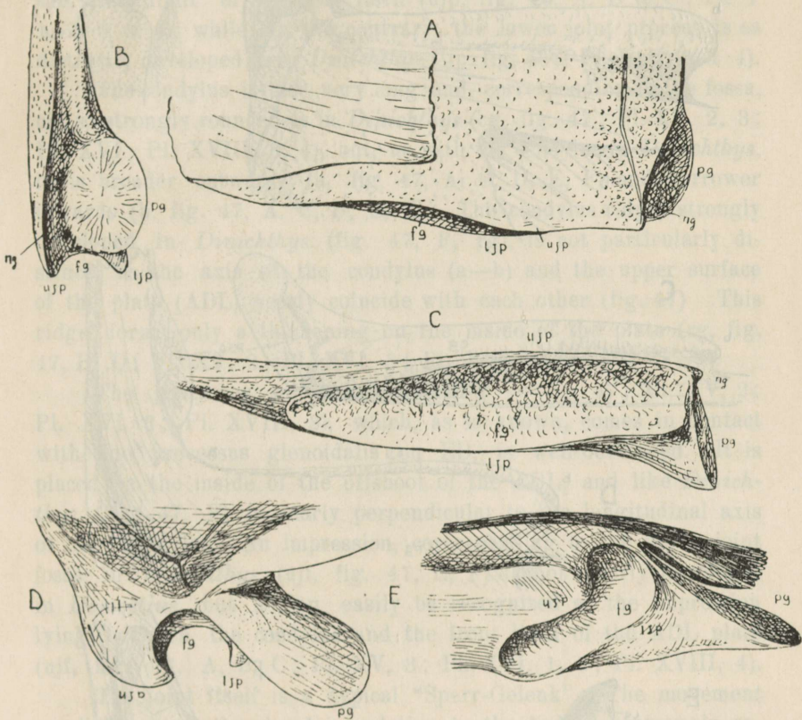
Fig. 46. Fossa condylus in Homostius (A, B, C) compared with that in Dinichthys (D & E, after Heintz, 1932, 2) A and D from outside, B — from side, C and E — from underside, fg — fossa condylus (fossa glenoidalis) fjp — lower joint process, ng — small protuberated ridge, pg — processus glenoidalis, ujp — upper joint process.
