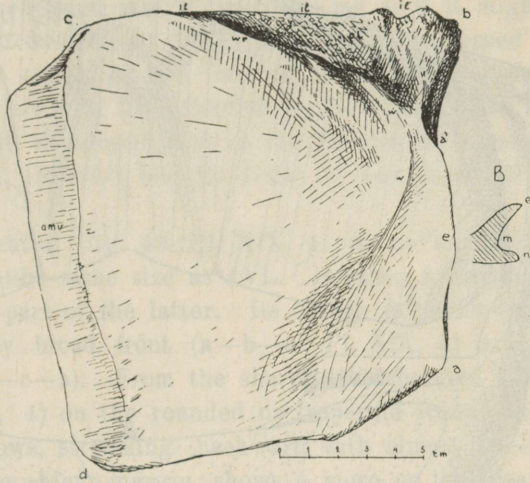
Fig. 42. The inner view of the antero-ventro-lateral plate (A) and cross-section of the outside margin (B). a-b — outside margin, a-e-a 1 — ridge on the outside margin, al — overlapping margin covered by the hind wing of the AL plate, amv — overlapping margin covering the AMV plate, b — thickened, protuberated outside front angle, b-c — front margin, c-d — inside margin, d-a — hind margin, il-il — part of the front margin, where the inside of the IL plate comes in contact with the AVL plate. m — groove along the outside margin, n — the lower outside margin, w-w-wr — the ridge on the front margin of the plate, wr — the thickenings on the front margin.
