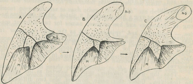
Fig. 50. The sub-orbital plates in three different groups of Homostius . A — Spitsbergen group ( H. arcticus ), B — Baltic group ( H. latus ) and C — Scotch group ( H. milleri ).
