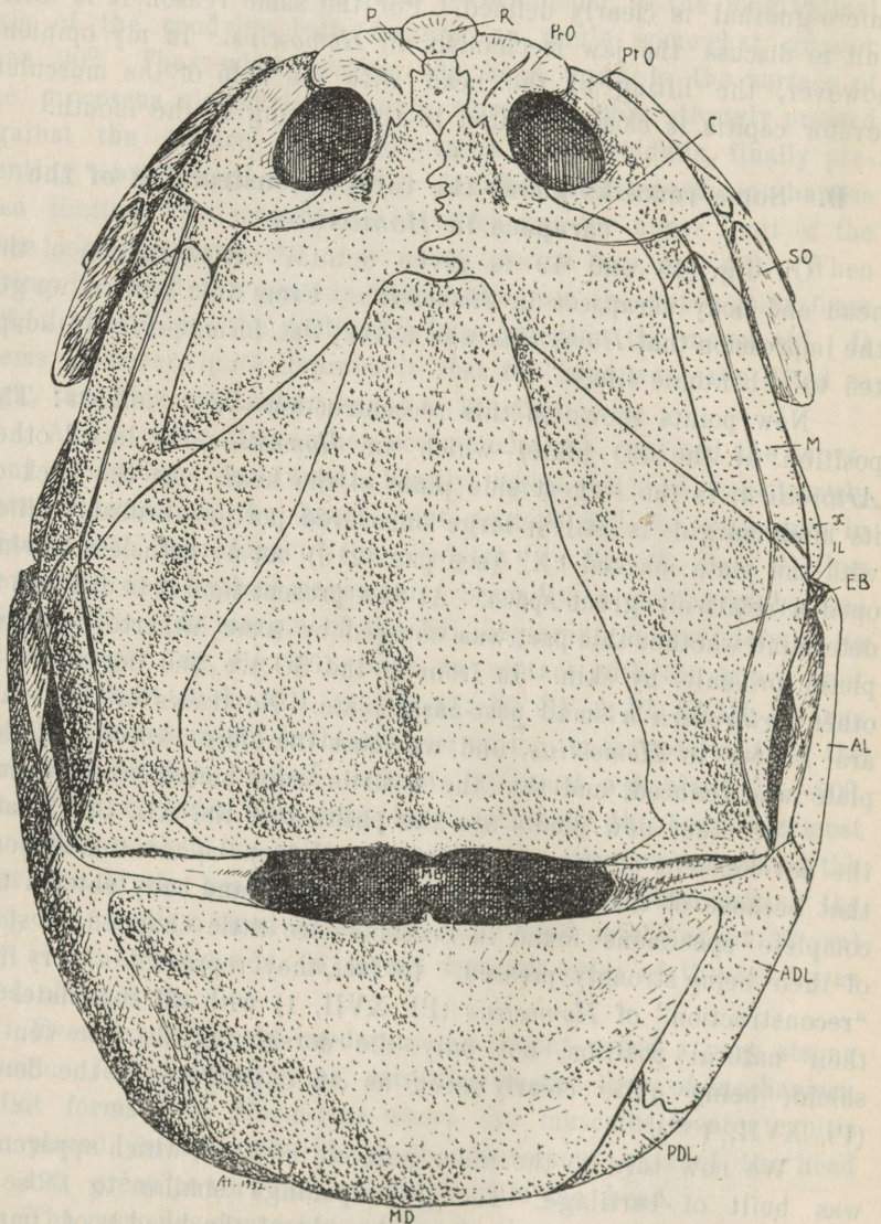
Fig. 48. The reconstruction of the head and body carapace of Homostius sulkatus Kut. from above. Explanation as in fig. 1 and fig. 43.
