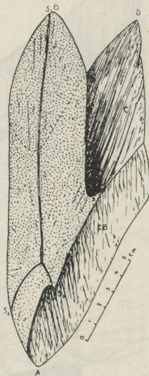
Fig. 12. The left marginal plate figured from the outside. A — posterior point, B — upper outside point, C — margin overlapped by C , D — upper inside point, EB — margin overlapped by EB , s_1-s_2-s_3 — sensory canals, x — protuberated part of the tuberculated surface.
