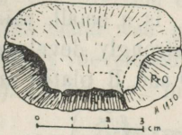
Fig. 21. The rostral plate from the outside. PrO — overlapping margin covered by the PrO plate. R — cavity, where the protuberated front part of the P plate fits in.
