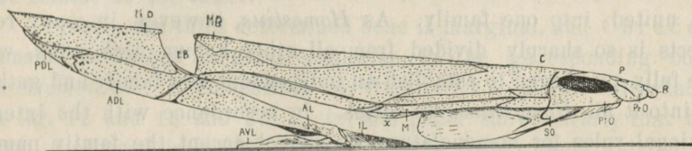
Fig. 49. The same reconstruction seen from the right side. Explanation as in fig. 1 and fig. 43.
