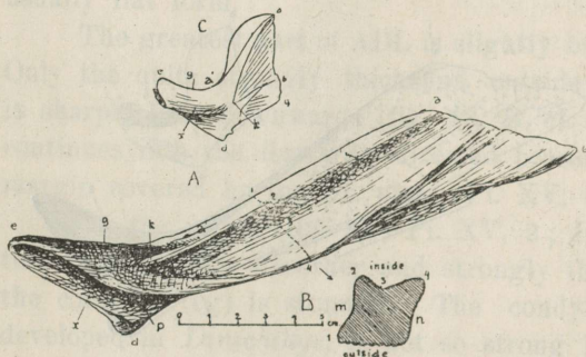
Fig. 38. The antero-lateral plate of Homostius sp. viewed from the inside (A) and in cross-section. (B) compared with the corresponding plate of Dinichthys sp. (C, strongly reduced) a-a' — ridge in front of the overlapping margin, a-k-b — overlapping margin covering the ADL plate. e-p — impression on the underside of the hind wing. m — front margin of the ridge, n — hind margin of the ridge. Rest as in fig. 37.
