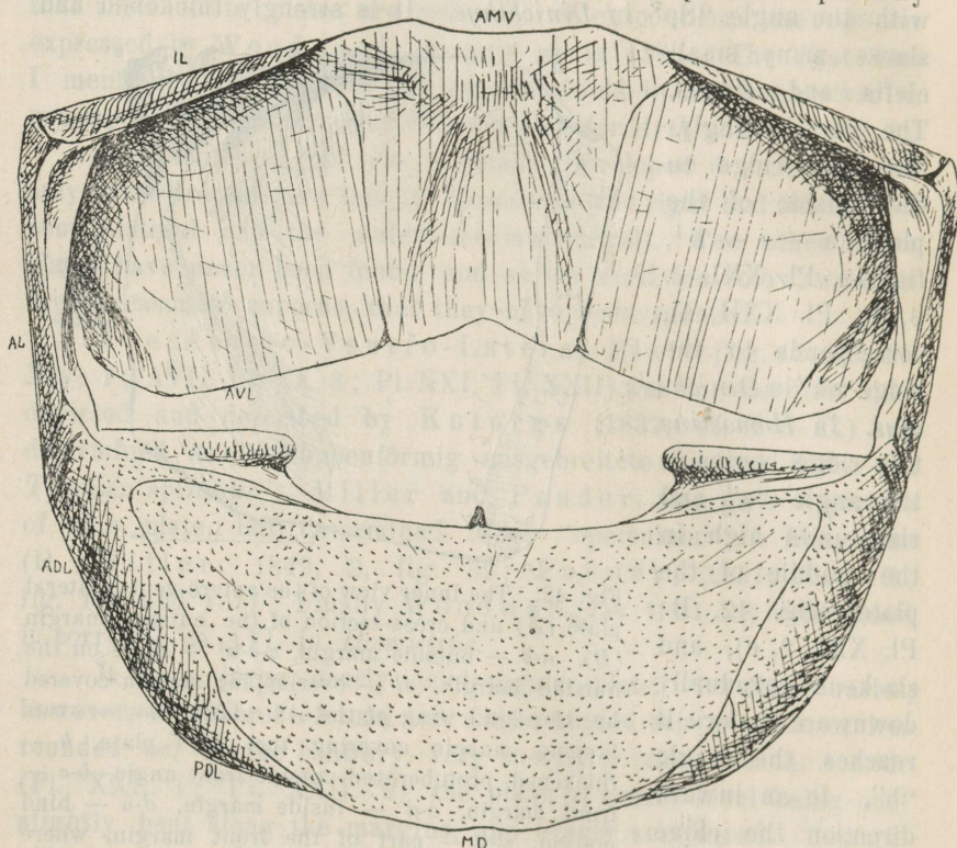
Fig. 43. The reconstruction of the body carapace of Homostius sulcatus Kut. seen from above. ADL — antero-dorso-lateral plate, AL — antero-lateral plate, AMV — antero-median-ventral plate, AVL — antero-ventro-lateral plate, IL — intero-lateral plate, MD — median-dorsal plate, PDL — postero-dorso-lateral plate.
