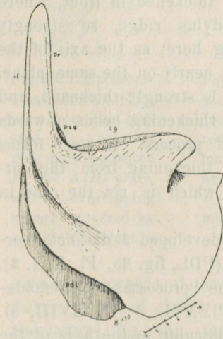
Fig. 35. The antero-dorso-lateral plate of Homostius sp. viewed from the inside. pdl — overlapping margin, which covered the PDL plate, psg — processus-subglenoidalis. Rest as in fig. 33.
