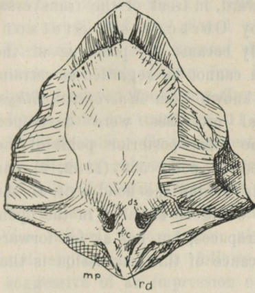
Fig. 8. The median-basal plate of Coccosteus sp. from Sjøass (Traut-schold) from the inside. Explanation as in fig. 5.
