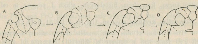
Fig. 51. Possible change of the front part of the head roof in the development line Acanthaspis — Homostius . A — Jaekelaspis solnördali Htz, from Spitsbergen. B — Homostius arcticus Htz. C — Homostius latus A sm. D — Homostius milleri Trq.
