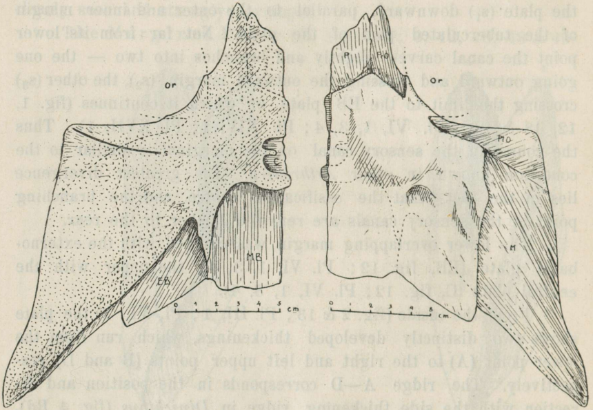
Fig. 14. The left central plate seen from the outside. C — overlapping margin covered by adjoining right C plate, EB — overlapping margin covered by the EB plate, MB — the same covered by the MB plate, Or — margin of the orbital opening, s-s — sensory canal.
