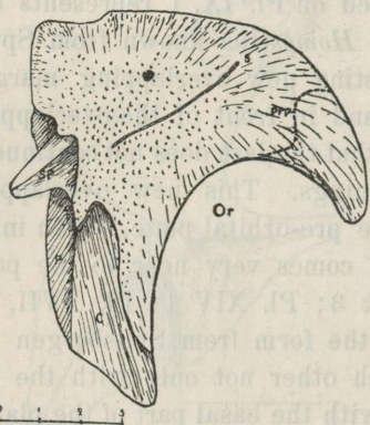
Fig. 18. The right pre-orbital plate seen from the outside. C margin overlapped by the C plate. Or — position of the orbital opening, P — margin overlapped by the P plate, prp — pre-orbital process, s — sensory canal, Sp — spine fitting into the cavity on the upper part of the P plate.
