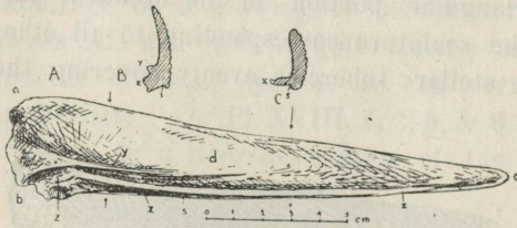
Fig. 41. The inter-lateral plate from the inside (A) and two cross sections of it (B & C), a-d-b — thin part overlapping the hind wing of the AL plate. s — step under the ridge x-x. x-x — lower ridge, z — thickened hind part, z-y — upper ridge.
