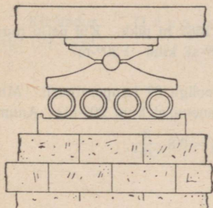
Joon. 50. Metallsilla rulltoed.
