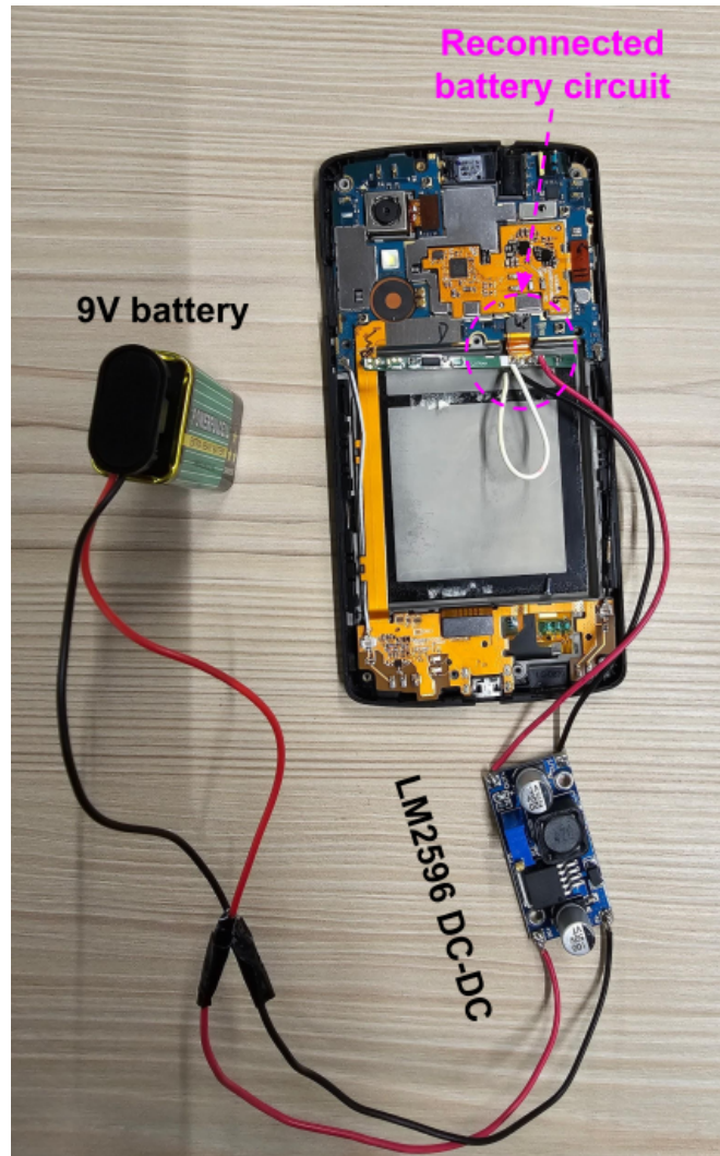
Figure 4.1: This figure illustrates the battery circuit modification for the Nexus 5, which enables the phone to run on a 9V battery.
