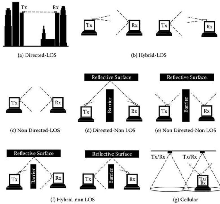
Figure 5. Different configurations of wireless IR links [19].
