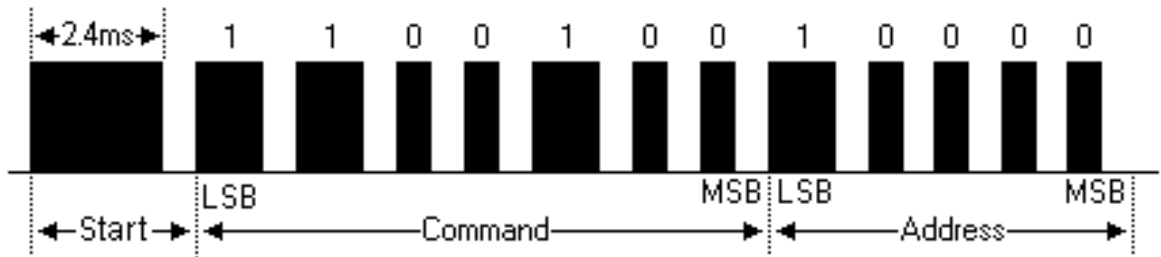
Figure 11. Example pulse stream of a 12-bit SIRC encoded message [29].
