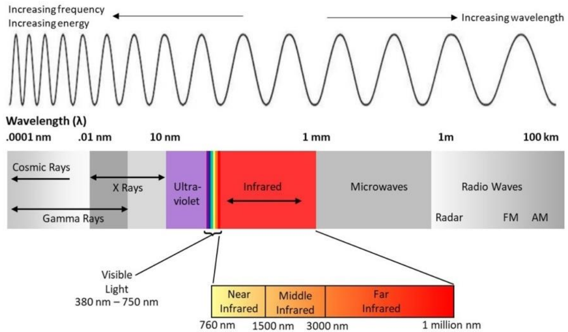
Figure 2. A representation of the electromagnetic spectrum including the infrared light broken down to three sections [5].
