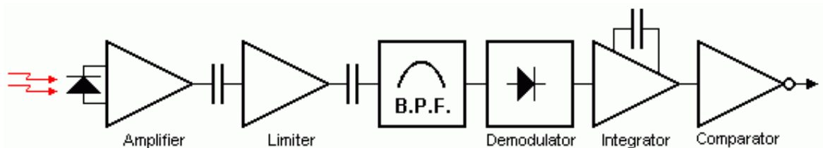
Figure 7. A typical block diagram of an IR receiver [25].
