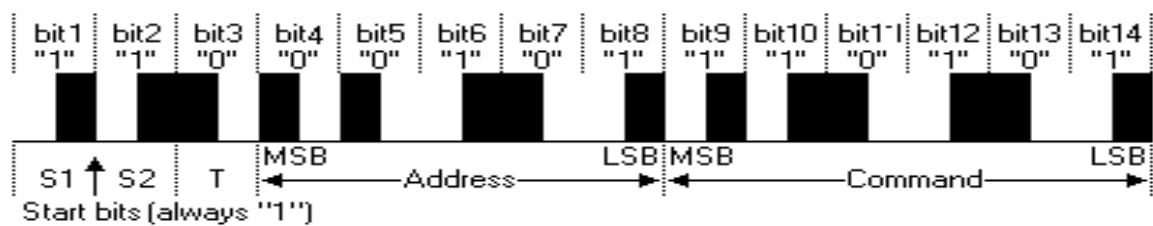
Figure 13. Example pulse stream of a RC-5 encoded message [31].
