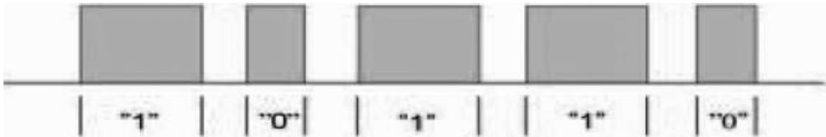
Figure 10. Pulse-length coding [23].
