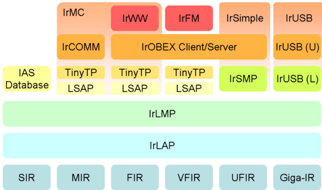
Figure 5. The IrDA protocol stack layers [20].
