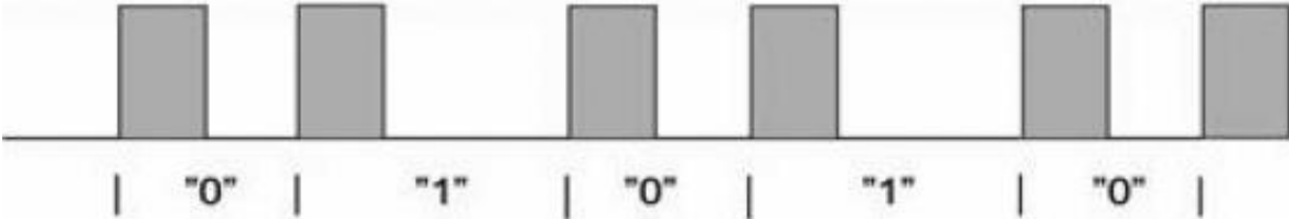
Figure 8. Pulse-distance coding [23].
