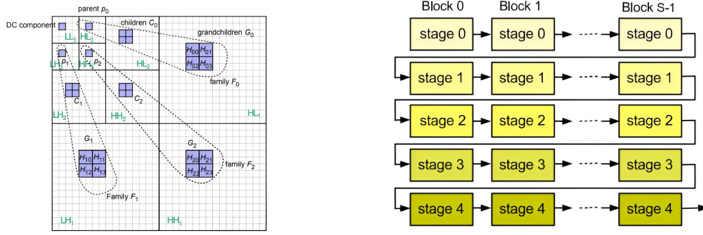
(a) "Schematic of Wavelet-Transformed Image" [3].
