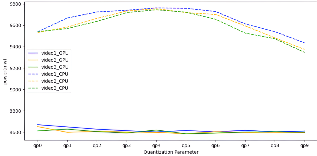
Figure 10. H.264 Graph of the evolution of the mean Power consumption compared to the change in the quantization parameter.
