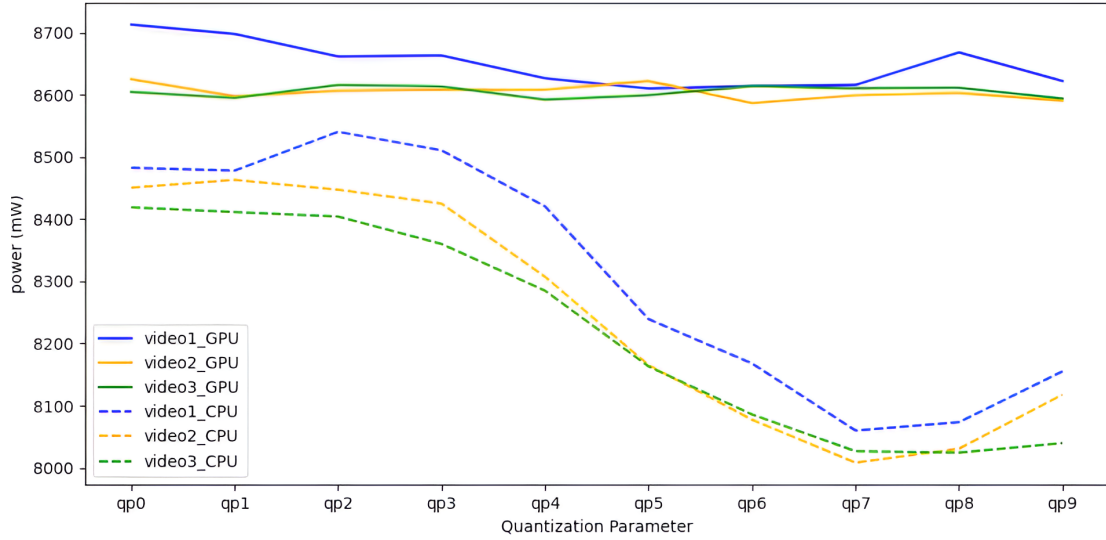
Figure 14. H.265 Graph of the evolution of the mean Power consumption compared to the change in the quantization parameter.
