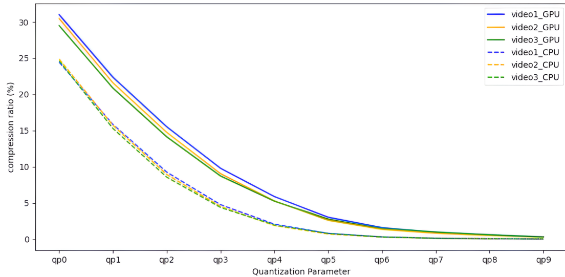
Figure 7. Graph of the evolution of the compression ratio compared to the change in the quantization parameter.
