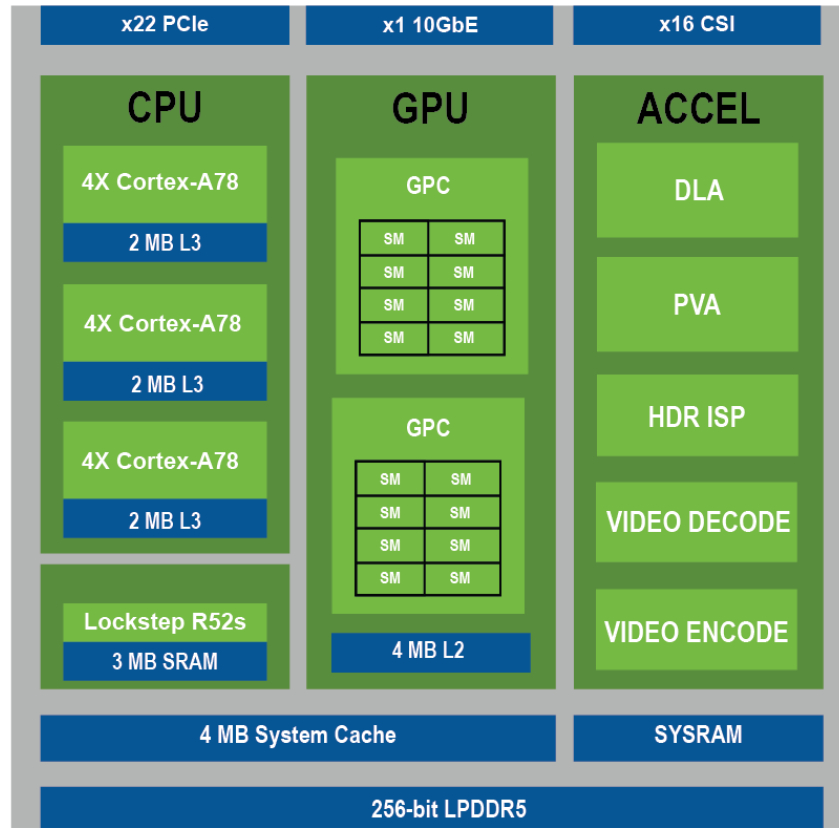
Figure 3. "Orin SoC Block Diagram" [2].
