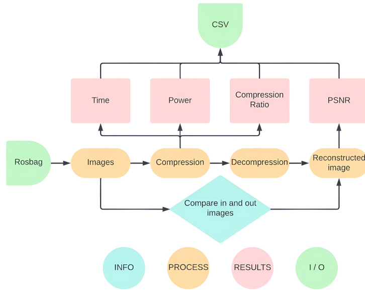
Figure 6. "Overview of the benchmark process".
