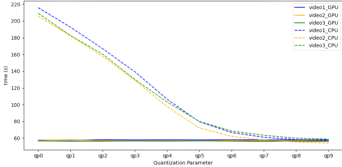
Figure 8. Graph of the evolution of the execution time compared to the change in the quantization parameter.
