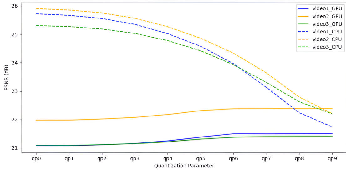
Figure 13. Graph of the evolution of the PSNR image quality compared to the change in the quantization parameter.
