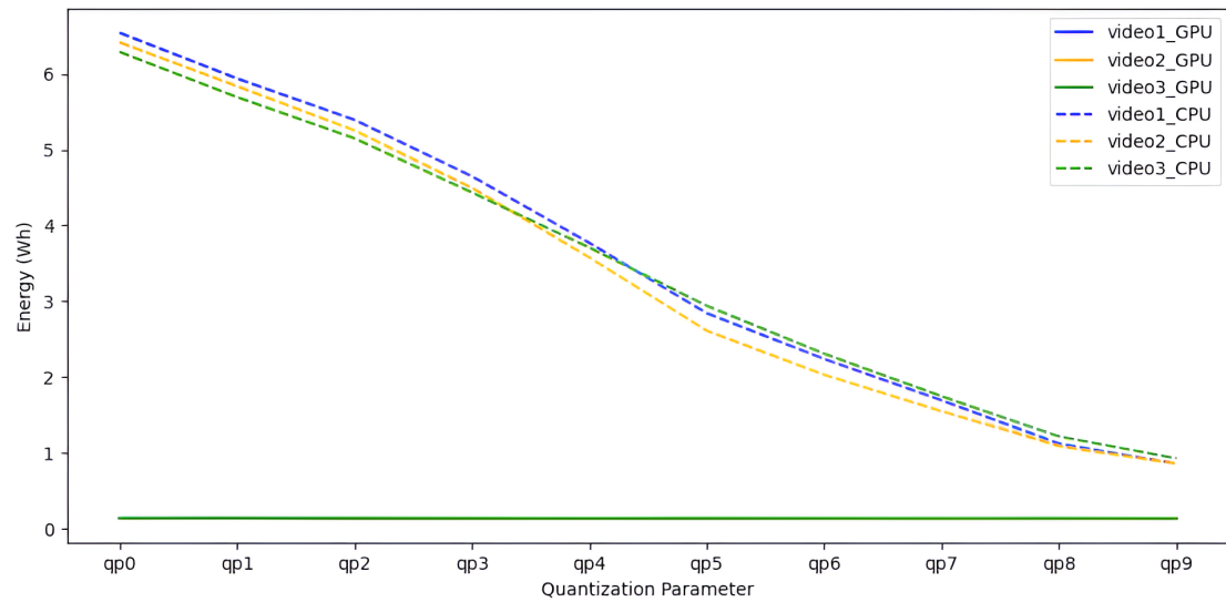
Figure 18. H.264 Graph of the evolution of the Energy consumption compared to the change in the quantization parameter.
