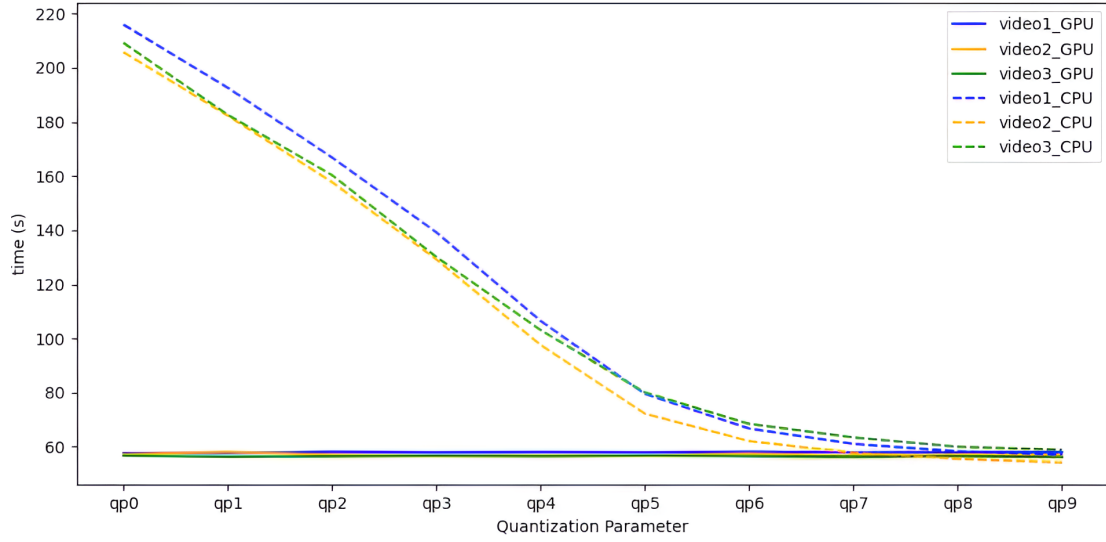
Figure 12. Graph of the evolution of the execution time compared to the change in the quantization parameter.
