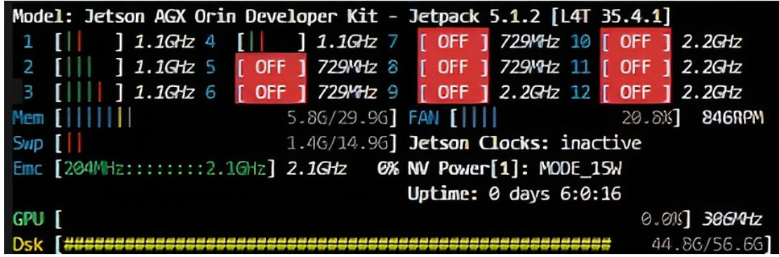
Figure 15. JTOP panel showing no GPU use while running CompressAI models
