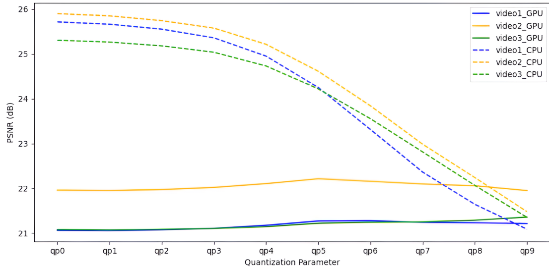
Figure 9. Graph of the evolution of the PSNR image quality compared to the change in the quantization parameter.
