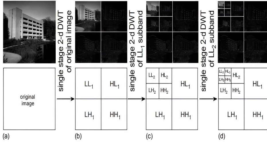
Figure 4. " Three-Level 2-d DWT Decomposition of an Image" [3].
