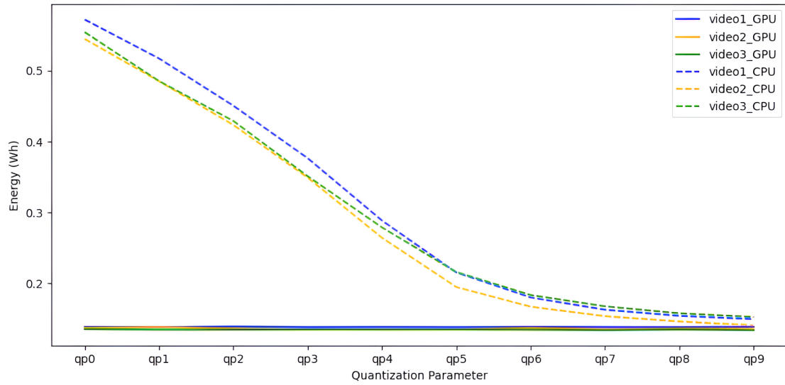
Figure 17. 265 Graph of the evolution of the Energy consumption compared to the change in the quantization parameter.
