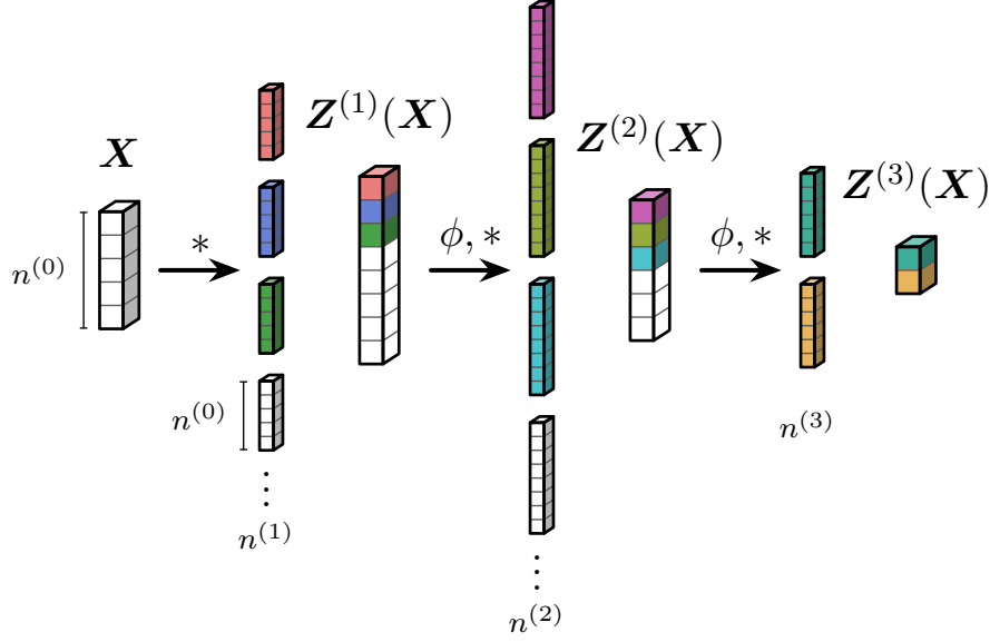
Figure 1: An example of a fully connected neural network with L = 3 layers. Each fully colored rectangle represents a row W^{(\ell)}[i, :] of the weight matrix W^{(\ell)} , visualized as a vertical bar, where the color is different for each i \in \llbracket n^{(\ell+1)} \rrbracket . The information flows through the network as follows. For each row of W^{(0)} , we compute the inner product between the row of W^{(0)} and the input X \in \mathbb{R}^{n^{(0)}} , then add the bias term to the result. This produces the output of a single neuron in the next layer (shown with the same color as the weight row). Performing this n^{(1)} times and collecting the results into a vector gives us Z^{(1)} . We then apply the activation \phi and repeat the process.
