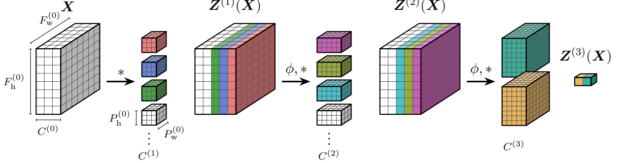
Figure 2: An example of a deep convolutional neural network inspired by Garriga-Alonso and Wilk (2021). This network has D = 2 spatial dimensions and L = 3 layers. Each colored cube represents the weight slice W^{(\ell)}[i, :, :] , where the color is different for each i \in \llbracket C^{(\ell+1)} \rrbracket . The information flows through the network as follows. The input X \in \mathbb{R}^{C^{(0)} \times F_h^{(0)} \times F_w^{(0)}} is divided into possibly overlapping patches of size \mathbf{P}^{(0)} = (P_h^{(0)}, P_w^{(0)}) . For each set of weights W^{(0)}[i, :, :] , we compute the inner product between the weights and all the patches, then add the bias term to the result. This produces one slice along a single channel in the next layer (shown with the same color as the weights). Performing this C^{(1)} times for all sets of weights and concatenating the results gives us Z^{(1)} . We then apply the activation \phi and repeat the process.
