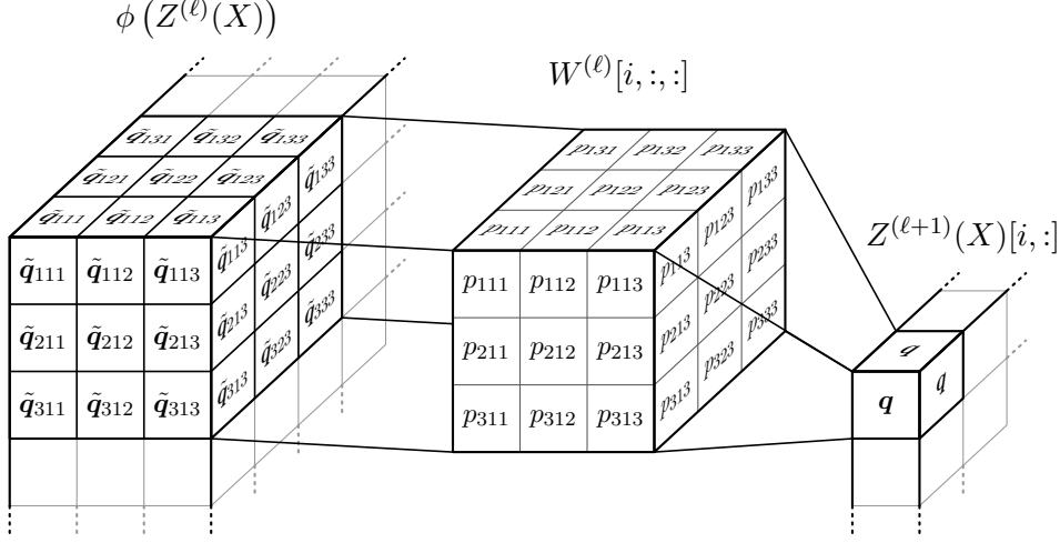
Figure 3: Consider an example where D = 2 , \mathbf{P}^{(\ell)} = (3, 3) and C^{(\ell)} = 3 . As a notational shorthand, write p_{abj} = (a, b, j) and \tilde{q}_{abj} = (\tilde{q}(a, b), j) , where a, b, j \in \llbracket 3 \rrbracket . Here (a, b) \in \llbracket \mathbf{P}^{(\ell)} \rrbracket is patch index and j is a channel index. Given an output position \mathbf{q} in layer \ell + 1 and a patch index \mathbf{p} , the patch function returns the corresponding spatial position \tilde{q}(\mathbf{p}) in layer \ell . As \mathbf{p} varies over \llbracket \mathbf{P}^{(\ell)} \rrbracket the function traces out the patch in the input. The same weight W^{(\ell)}[i, :, :] is used for each \mathbf{q} \in \llbracket \mathbf{F}^{(\ell+1)} \rrbracket to produce the elements of Z^{(\ell+1)}(X)[i, :] .
