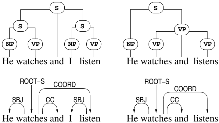
Figure 3: Parse trees of coordination examples.
