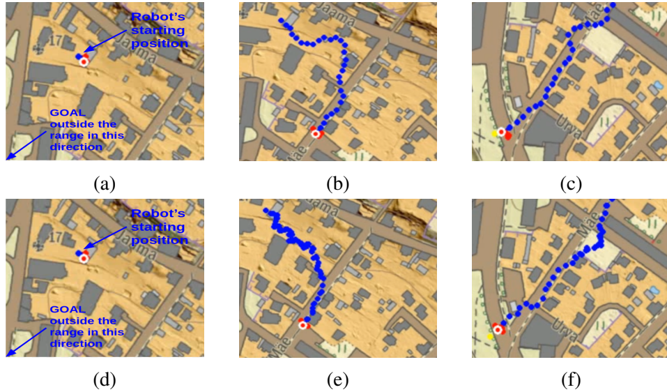
Figure 5.9: Robot trajectories for raster map simulation scenario 2: Initializing the robot relatively farther than in scenario 1 and recording the behavior shown by naive approach- (a), (b) and (c), trajectory followed by physical A*- (d), (e) and (f) taken from simulation videos: video 10 and video 11
