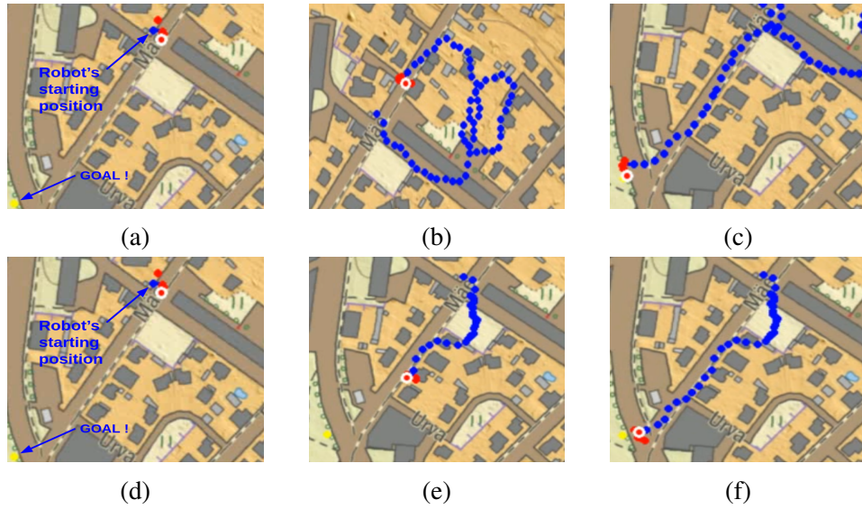
Figure 5.8: Robot trajectories for raster map simulation scenario 1: Initializing the robot in the same place, behavior shown by naive approach- (a), (b) and (c), trajectory followed by physical A*- (d), (e) and (f), taken from simulation videos: video 8 , video 9
