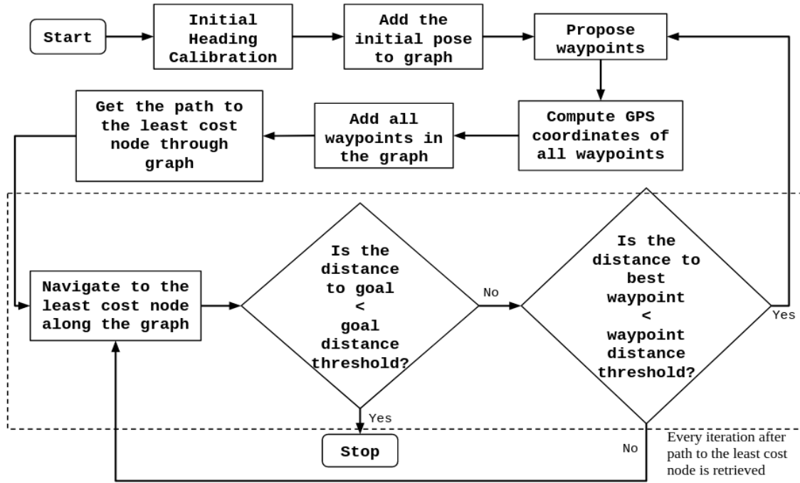
Figure 4.1: General workflow architecture.
