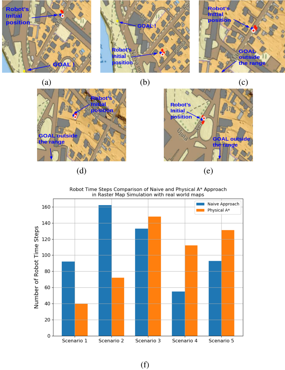
Figure 5.10: Quantitative analysis of raster map simulation: Starting location of robot in five different scenarios for quantitative analysis (a) to (e) taken from raster map simulation videos 12 , and the number of robot timesteps taken by the naive and physical A* implementations in corresponding scenarios (f)
