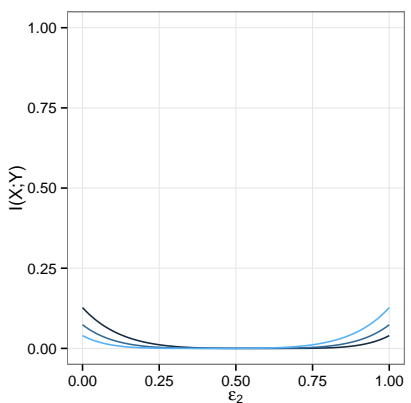
(b) \epsilon_1 = 0.4, 0.5, 0.6
