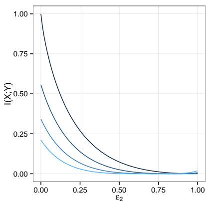
(a) \epsilon_1 = 0, 0.1, 0.2, 0.3
