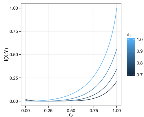
(c) \epsilon_1 = 0.7, 0.8, 0.9, 1
