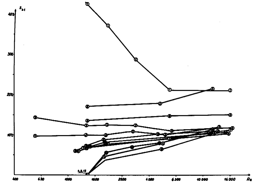
FIGURE 21.6. Turbulent dispersion of mobilities. The type of nozzle (Figure 21.1) and the value of the ratio l'/r_2 (in parentheses) are given for the respective curves:
