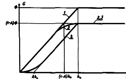
FIGURE 24.1. Function G of an integral counter:
