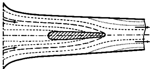
FIGURE 4.1. Flow lines in the measuring capacitor: - - - - - flow lines; ——— boundary surface; ····· flow lines on which q(k) = 0 ; - · - · - entrance surface.
