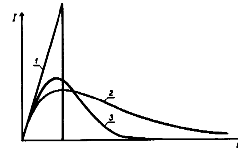
FIGURE 22.2. Characteristics of a differential counter: 1—laminar flow; 2—complete mixing; 3—according to experimental results.
