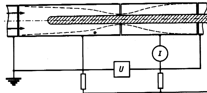
FIGURE 9.1. Example of a measuring capacitor in which the normal conditions are not satisfied.
