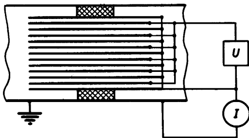
FIGURE 11.1. Gunn filter.
