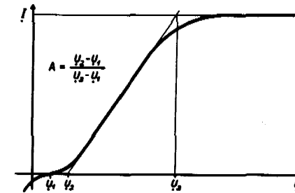
FIGURE 24.2. Determination of the relative adsorption from the characteristics of an integral counter with an outer collector plate:
