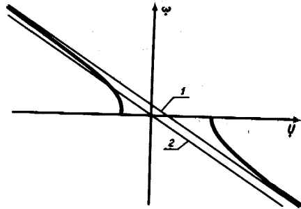
FIGURE 16.2. Dependence \omega = 1/k_0 on voltage: 1— asymptote of the function \omega(U) ; 2— \omega(U) for \phi = 0 .
