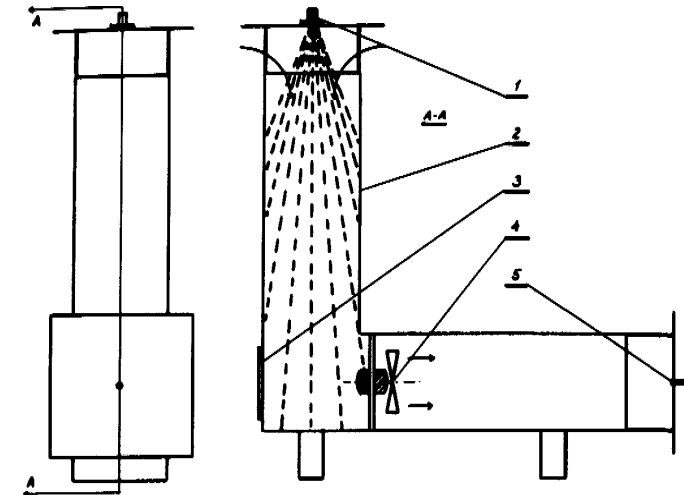
FIGURE 21.3. Ion generator. 1—preparation \text{Sr}^{90} (1.0 mCi); 2—air channel; 3—door; 4—fan; 5—measuring capacitor of the counter.
