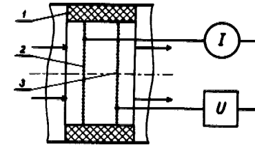
FIGURE 6.3. Counter in which air is blown through grids:
