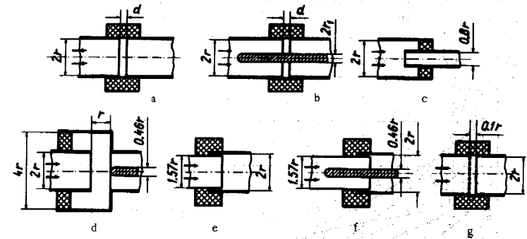
FIGURE 15.4. Entrance arrangements.
