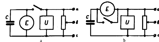
FIGURE 25.1. Principal circuit arrangements of a counter:
