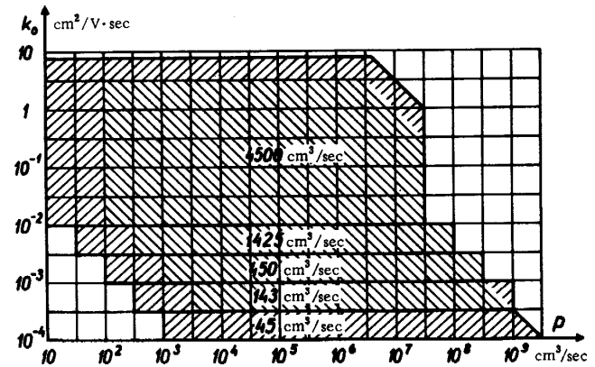
FIGURE 36.4. Measurement limits of the SAI-TGU-66 counter. The hatchings in the other direction correspond to the region in which marked distortions are possible.
