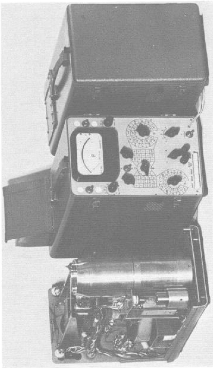
FIGURE 36.5. Three forms of the 8A1-TCU-66 counter (with cover removed, in working state, in portable state).
