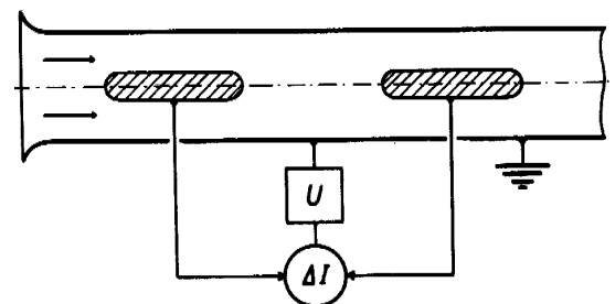
FIGURE 9.2. The counter of Imyanitov. \Delta I is the differential electrometer.
