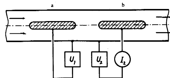
FIGURE 6.1. Counter with a precondenser:
