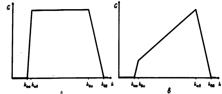
FIGURE 8.1. G -function of the second-order differential counter:
