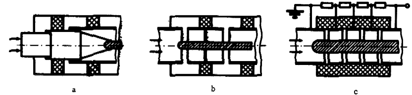
FIGURE 32.2. Electrostatic shields.
