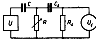
FIGURE 28.2. Circuit arrangement for the determination of s_{\tau U}(RC) :
