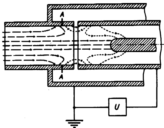
FIGURE 14.1. Example of a capacitor inlet: - - - - - flow lines; ····· flow lines for which \rho(k) = 0 ; A designates the separation region.
